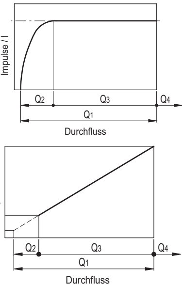
HVF-E (G3/8 - G1/2)
