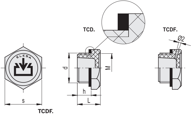
TCDF.
